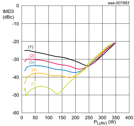
V_{DS} = 50 \text{ V}; f_1 = 860.0 \text{ MHz}; f_2 = 860.1 \text{ MHz}. (1) I_{Dq} = 600 \text{ mA} (2) I_{Dq} = 1000 \text{ mA} (3) I_{Dq} = 1300 \text{ mA} (4) I_{Dq} = 1600 \text{ mA} (5) I_{Dq} = 2000 \text{ mA}
