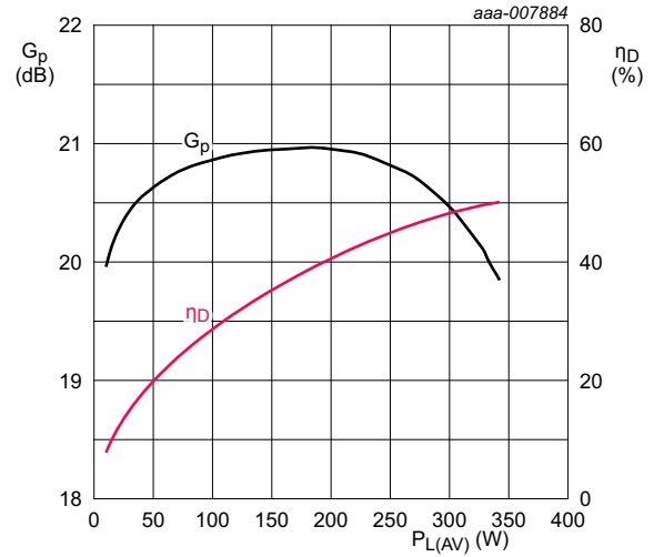
V_{DS} = 50 \text{ V}; I_{Dq} = 1300 \text{ mA}; f_1 = 860.0 \text{ MHz}; f_2 = 860.1 \text{ MHz}.
